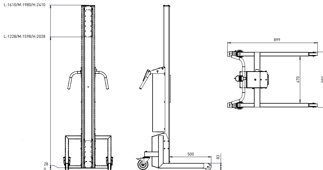
INOX 200 L/M/H - Standard setup: Leg 1 (Standard assembly if nothing is specified)
