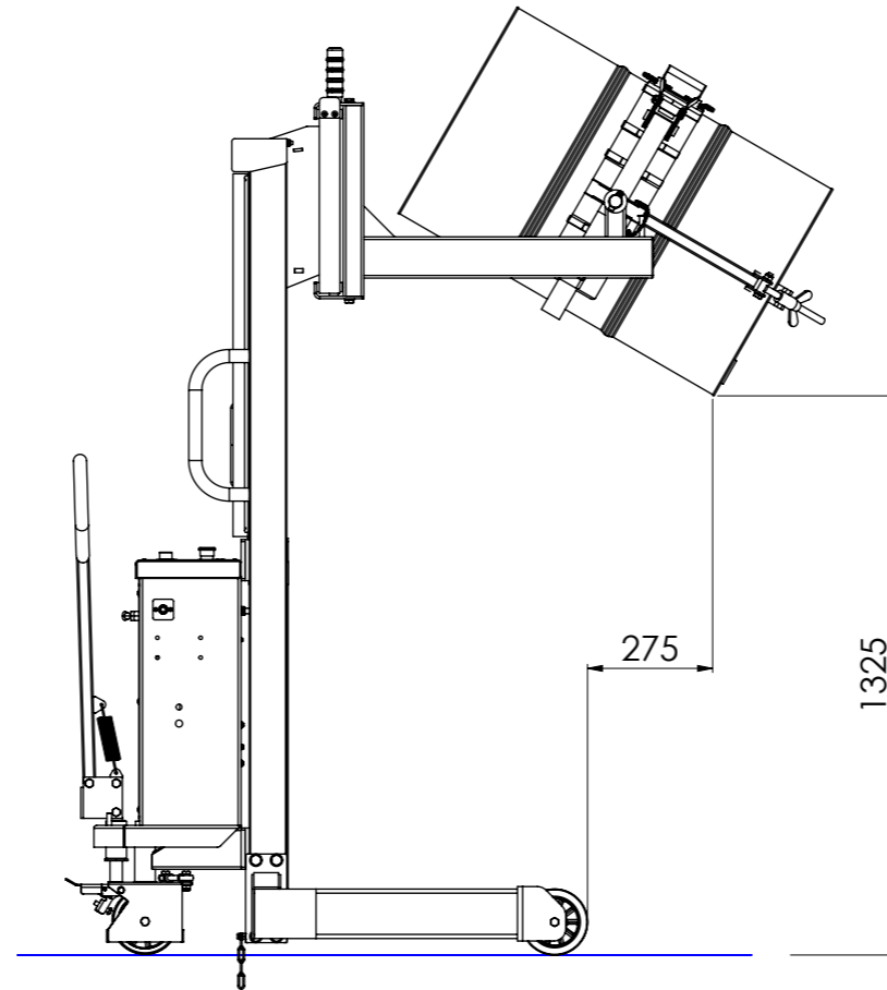
TIP OF 30°
